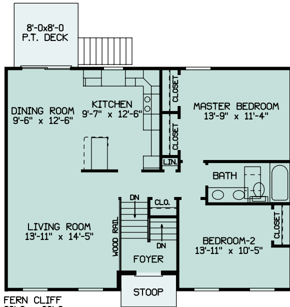
FERN CLIFF 36'-0" x 28'-0" 994 SQ. FT.
