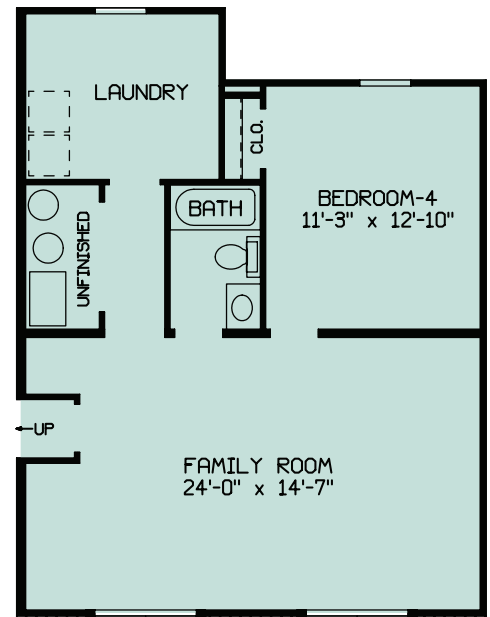
Covington Plan D 52' x 34' 2309 Sq. Ft.
