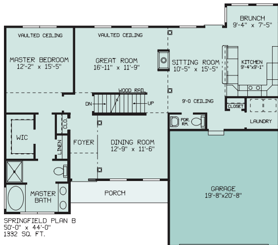
Springfield B 50' x 44' 1832 Sq. Ft.
