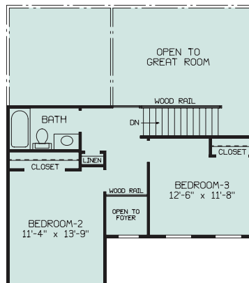
SPRINGFIELD PLAN B 30'-0" x 22'-0" 500 SQ. FT.
