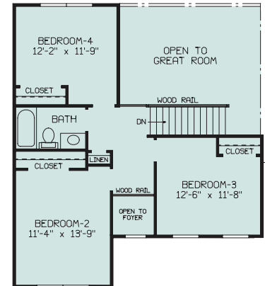
SPRINGFIELD PLAN B W/OPT. 4TH BEDROOM 30'-0" x 34'-0" 655 SQ. FT.
