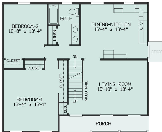
CATAWBA PLAN A & B - 36'-0" x 32'-0" - 1064 SQ. FT.
